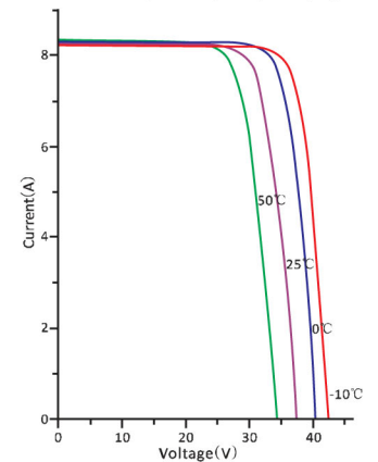
I-V Curves of PV Module at Different Cell Temperatures (AM1.5, 1000W/m 2 )
