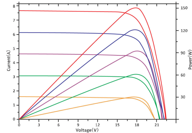
Current-Voltage & Power-Voltage Curve (150W)
